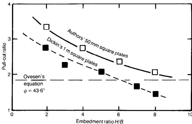
Fig. 14. Variation of pull-out ratio with embedment ratio
