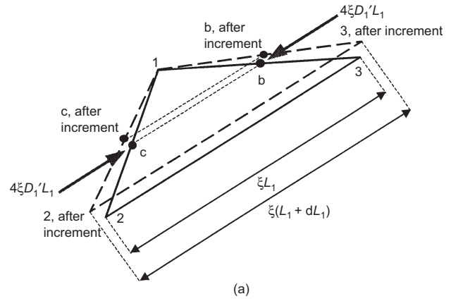
Fig. 14. Preliminary interpretations of triangular effective stresses. (a) forces 4\xi D'_1 L_1 acting on 123 due to the first triangular effective stress D'_1 .
