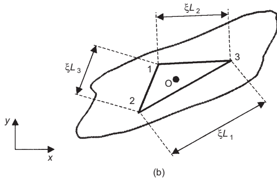
Fig. 3. Triangular representations of the same deformation. (a) Initial state. (b) Current state.
