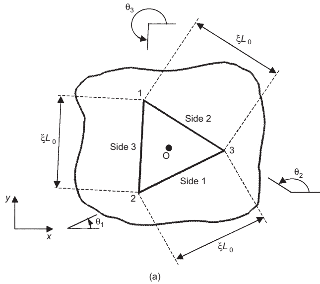
Fig. 14. Preliminary interpretations of triangular effective stresses. (a) forces 4\xi D'_1 L_1 acting on 123 due to the first triangular effective stress D'_1 .
