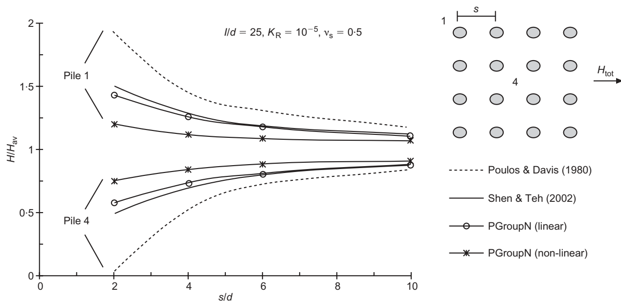
Fig. 13. Horizontal load distributions in a four-by-four fixed-head pile group
