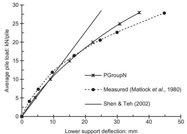
Fig. 11. Load–deformation behaviour for a five-pile group
