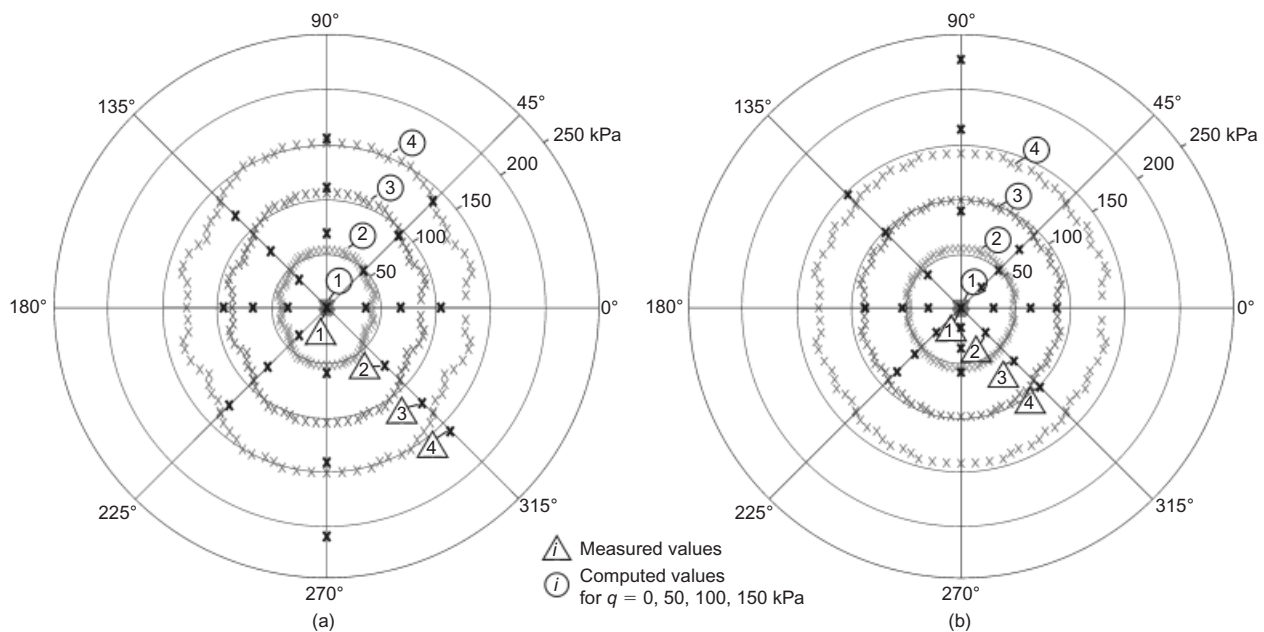
Fig. 17. Results of analysis B: (a) radial pressures on the pipe at r = 107 mm in the loose backfill; (b) radial pressures on the pipe at r = 107 mm in the compacted backfill
