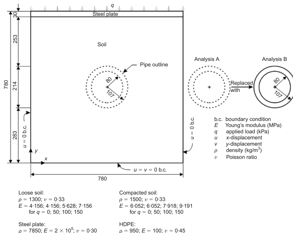
Fig. 16. FLAC model for analysis A and analysis B (all dimensions are in mm)
