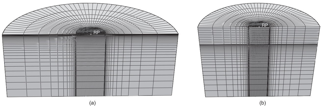
Fig. 5. FEA meshes for displacement probe and swipe tests: (a) surface foundation of diameter D (domain: 2.5D in depth and 3D in radius); (b) caisson foundation of diameter D and skirt length L = D (domain: 4.5D in depth and 3D in radius)
