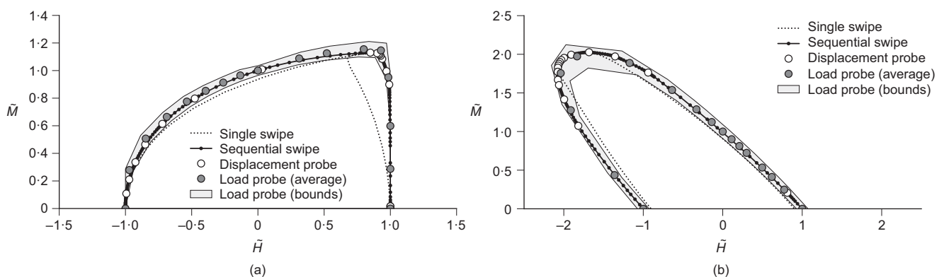
Fig. 9. Dimensionless HM failure envelopes: (a) surface foundation; (b) caisson foundation
