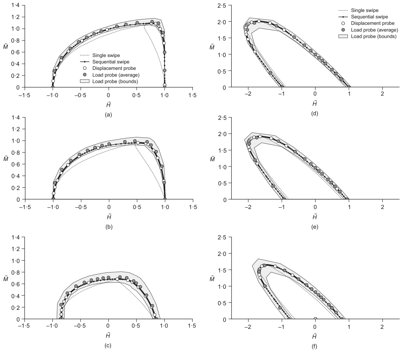
Fig. 10. Dimensionless HM failure envelopes at selected \tilde{V} levels for surface foundations: (a) \tilde{V} = 0.25 ; (b) \tilde{V} = 0.5 ; (c) \tilde{V} = 0.75 ; and caisson foundations: (d) \tilde{V} = 0.25 ; (e) \tilde{V} = 0.5 ; (f) \tilde{V} = 0.75
