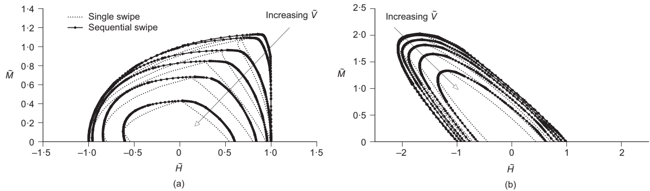
Fig. 11. Dimensionless HM failure envelopes at selected \tilde{V} levels ( \tilde{V} = 0, 0.25, 0.5, 0.625, 0.75, 0.85 ): (a) surface foundation; (b) caisson foundation
