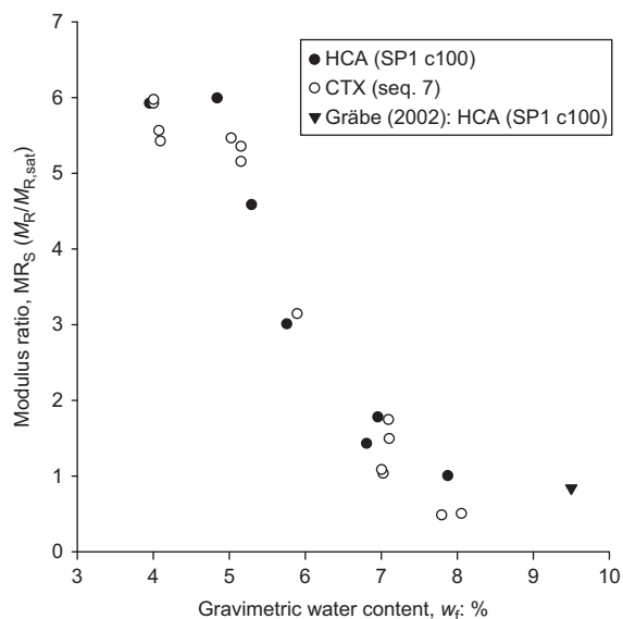
Fig. 6. Suction modulus ratio ( M_{R_s} ) indicating the relative change in M_R due to a change in water content (and associated suction) of the material. HCA and CTX M_R normalised by M_{R,sat} (HCA + 1v1). Value from Gräbe (2002) included for comparison only
