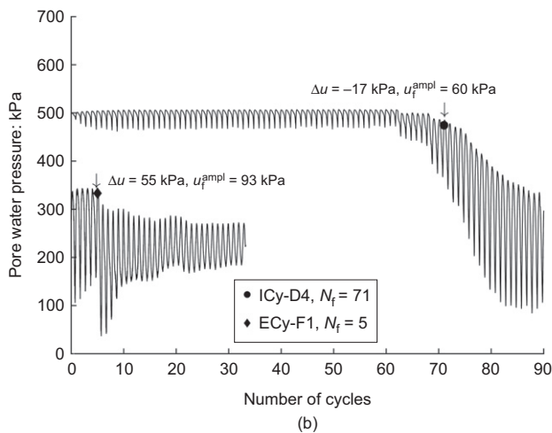
Fig. 10. (a) Cyclic axial strain and (b) pore water pressure trends for tests ICy-D4 and ECy-F1 performed at in situ and elevated stresses, denoting axial strains ( \epsilon_a ) and pore water pressure (PWP) at the end of the N_f cycle, and the PWP amplitudes ( u_f^{amp} ) of the N_f cycle
