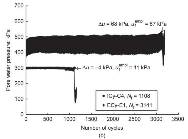
Fig. 11. (a) Cyclic axial strain and (b) pore water pressure trends for tests ICy-C4 and ECy-E1 performed at in situ and elevated stresses, denoting axial strains ( \epsilon_a ) and pore water pressure (PWP) at the end of the N_f cycle, and the PWP amplitudes ( u_f^{amp} ) for the N_f cycle
