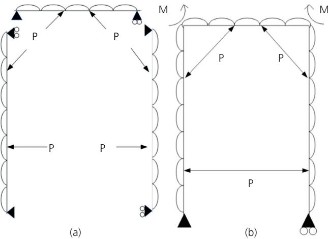
Figure 12. (a) Sketch showing current design philosophy for box retaining structures. Each wall is considered as a simply supported beam. (b) Possible alternative design philosophy for box retaining structures. Box behaves similarly to a portal frame, with the corners carrying moment
