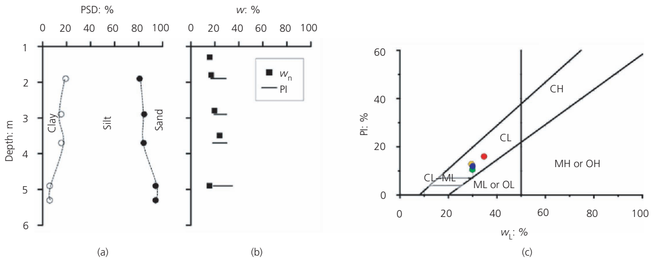
Figure 1. Soil classification at the installation site: (a) particle size distribution (PSD), (b) plasticity index and natural water content with depth and (c) Casagrande chart within the Unified Soil Classification System. C, clay; H, high plasticity; L, low plasticity; M, silt; O, organic
