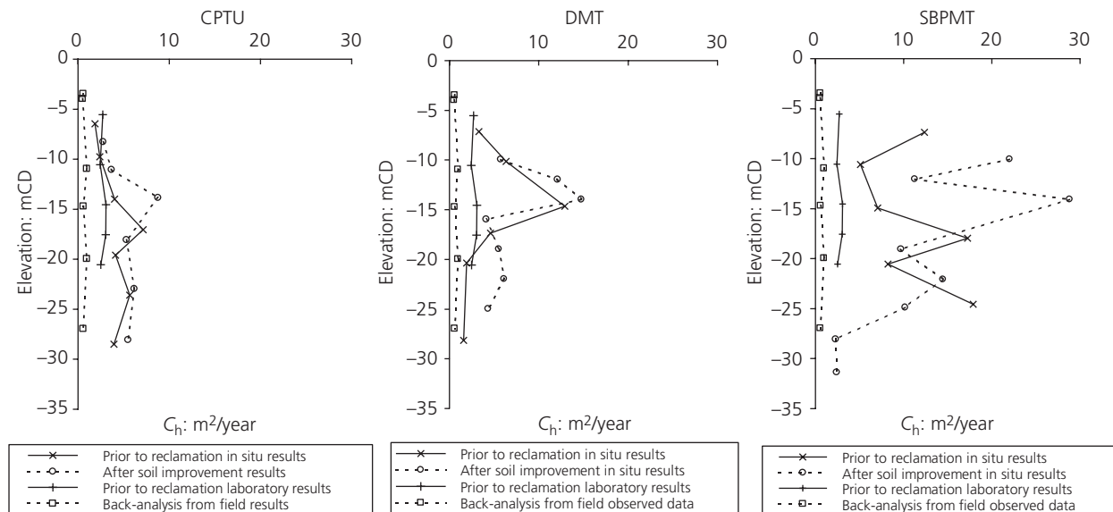
Figure 9. Coefficient of consolidation due to horizontal flow measured from in situ specialised tests
