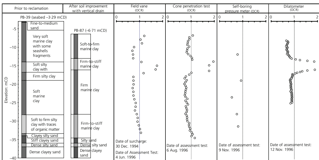
Figure 12. Degree of consolidation assessed using specialised in situ tests
