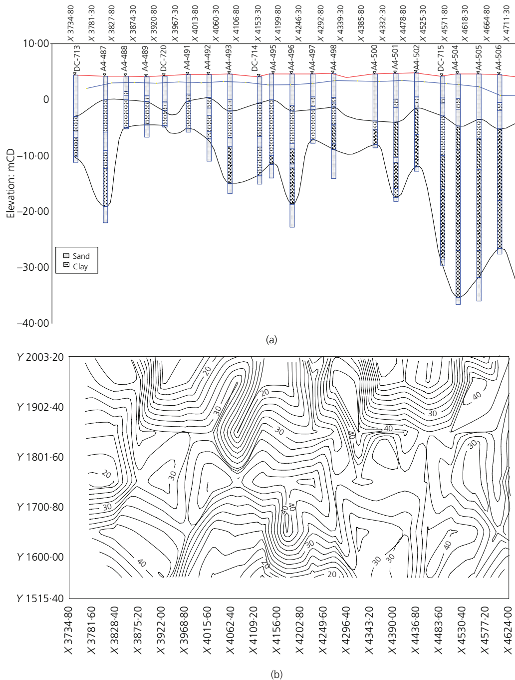
Figure 3. (a) Cross-section and (b) contours of proposed PVD installation depths. Distance in (a) and measurements in (b) are in metres
