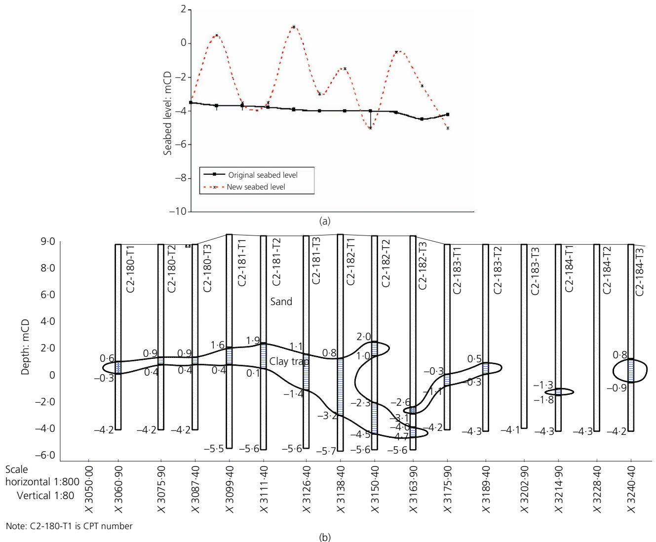
Figure 5. (a) Mud wave of seabed measured from CPTU tests. (b) Mud trapped measurements from CPTU tests
