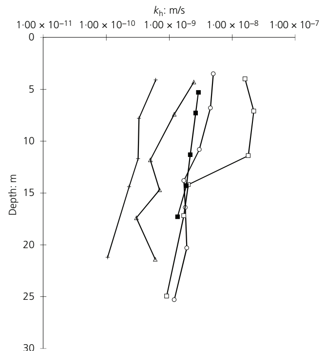
Figure 10. Horizontal hydraulic conductivity estimated from in situ specialised tests
