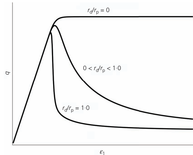
Figure 4. Modelling coupled plasticity-damage behaviour
