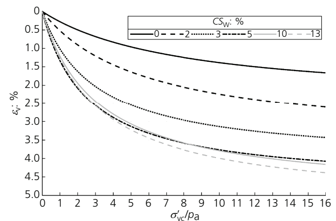
Figure 14. Hyperbolic regression curves from experimental data at different CS contents
