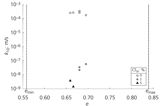
Figure 12. Hydraulic conductivity measurements on treated and untreated materials
