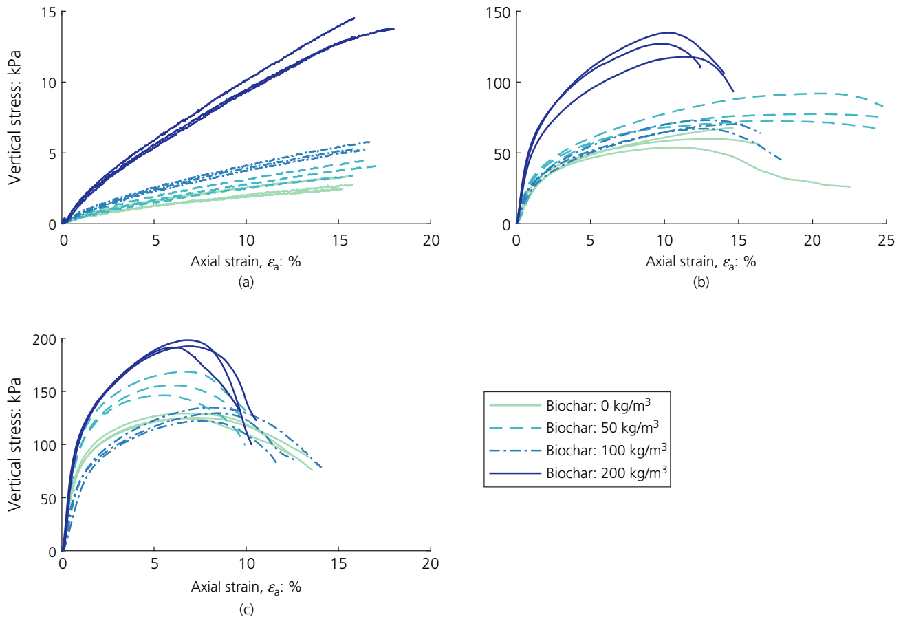
Figure 2. Stress–strain curves of the Tiller-Flotten peat stabilised with different levels of cement and biochar after 28 days of curing. Note the different scales on the vertical axes. Cement quantity: (a) 0 kg/m 3 , (b) 100 kg/m 3 (c) 200 kg/m 3
