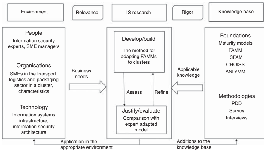
Figure 3. Research framework
