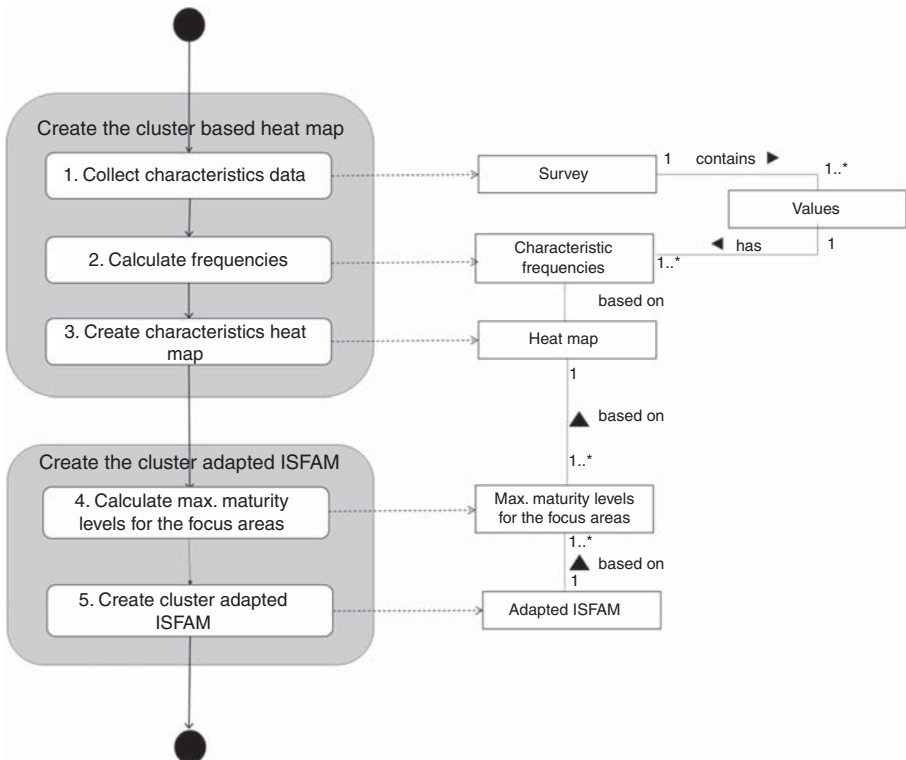
Figure 4. Method for Adaptive Information Security Maturity Modelling in Clusters (MAISMMC)
