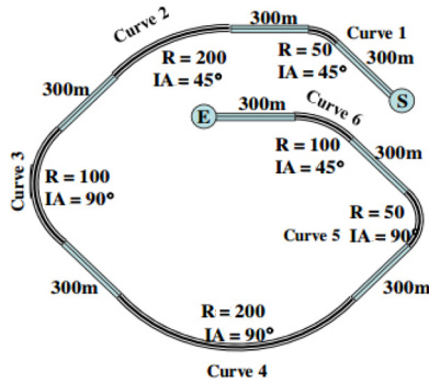
Figure 4 Driving route of experiments
