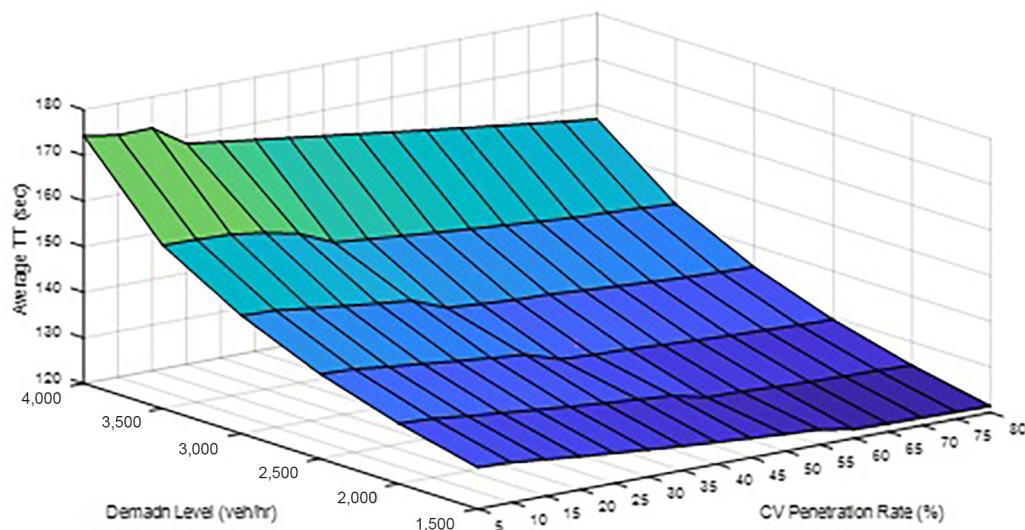
Figure 7 Freeway average travel time under different scenarios
