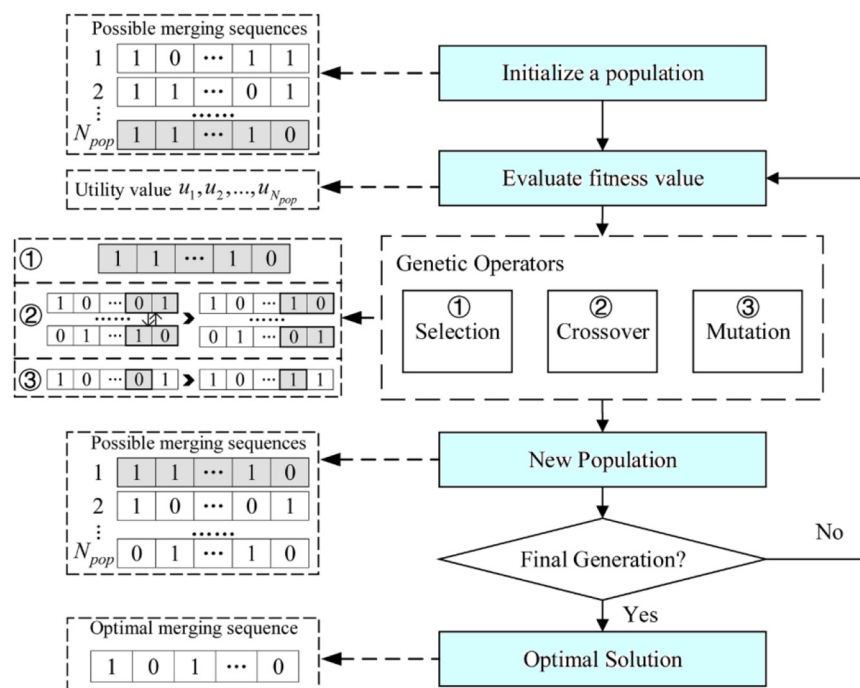
Figure 2 Merging sequence representation and flowchart of used genetic algorithm
