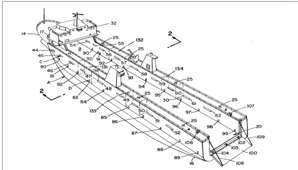
Figure 12. Semi-Submersible Stern-loading Vessel
