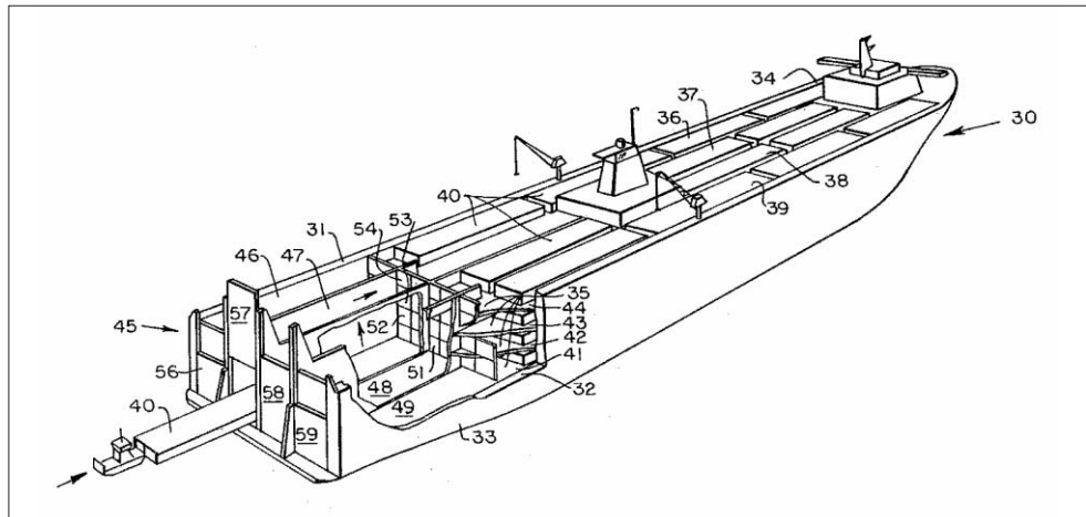
Figure 13. Semi-Submersible Stern-loading Barge Carrier Vessel
