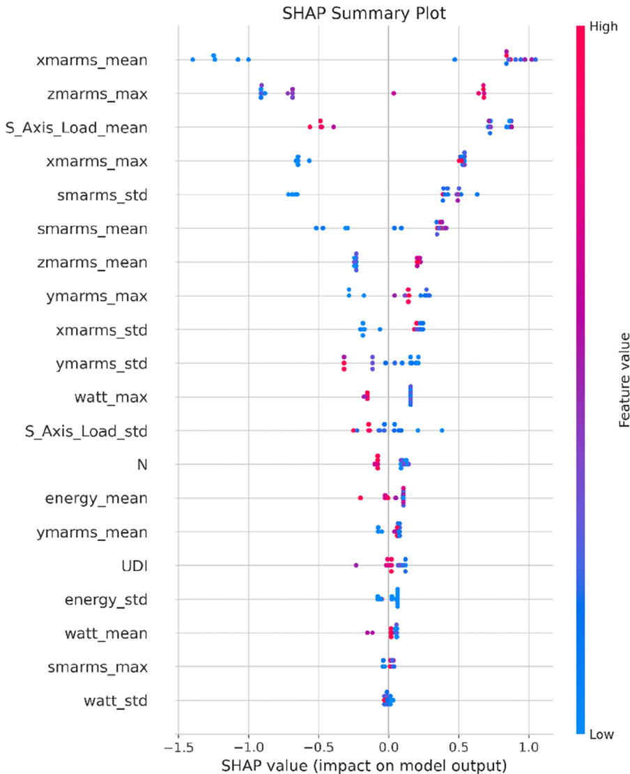
Figure 5. SHAP summary plot illustrating the contribution of individual features to anomaly prediction. Vibration-related variables, including xmarms_mean , zmarms_max , S_Axis_Load_mean , and smarms_std , exhibit the greatest influence on model output, confirming that machining anomalies are primarily governed by dynamic machine behaviour rather than nominal cutting parameters
