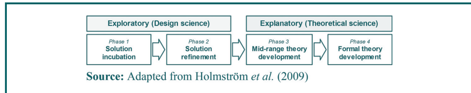
Figure 4 DSR approach
