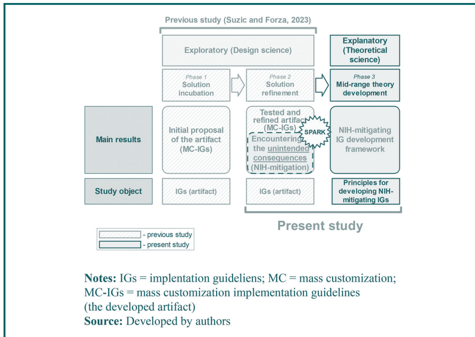
Figure 5 Research design
