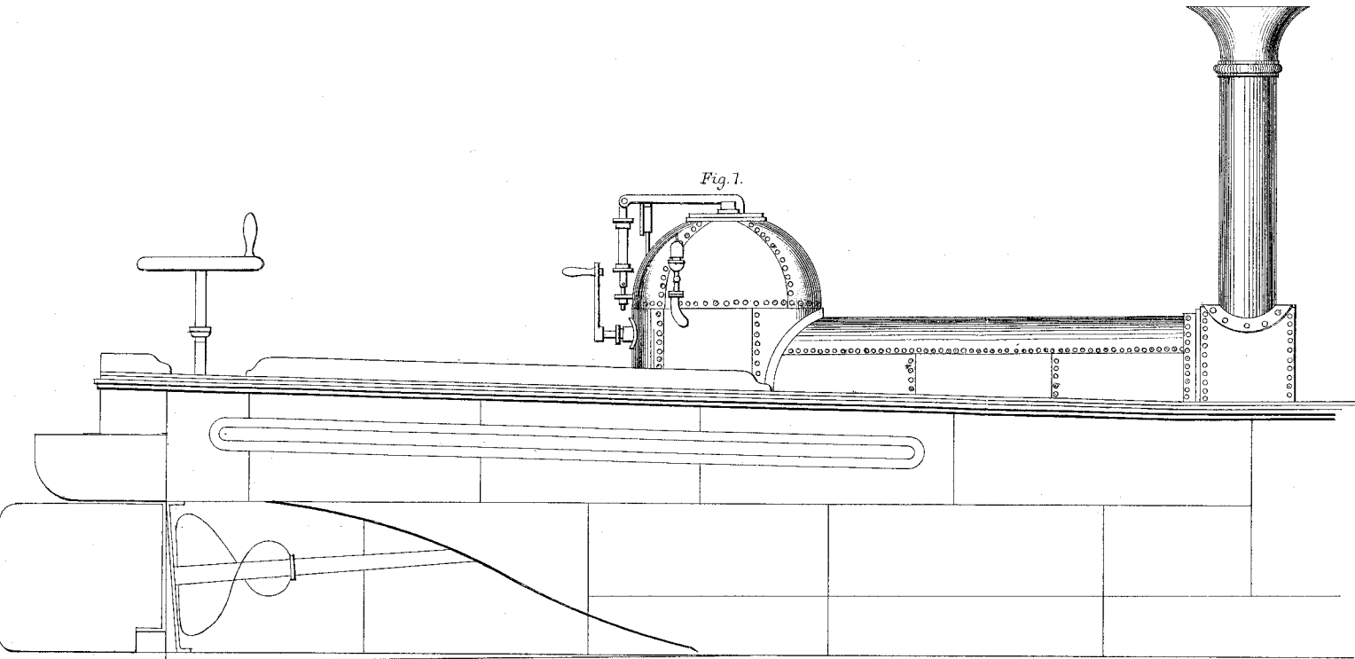
SIDE ELEVATION OF THE PIONEER.
