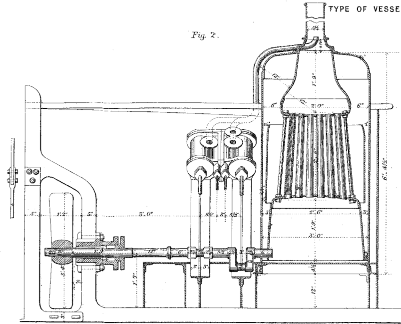
FRONT ELEVATION AND SECTION OF BOILER.
