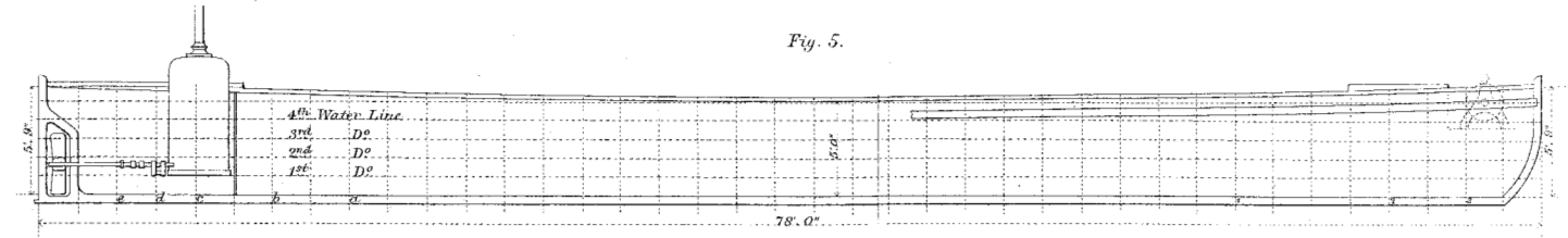
SECTIONAL ELEVATION.
