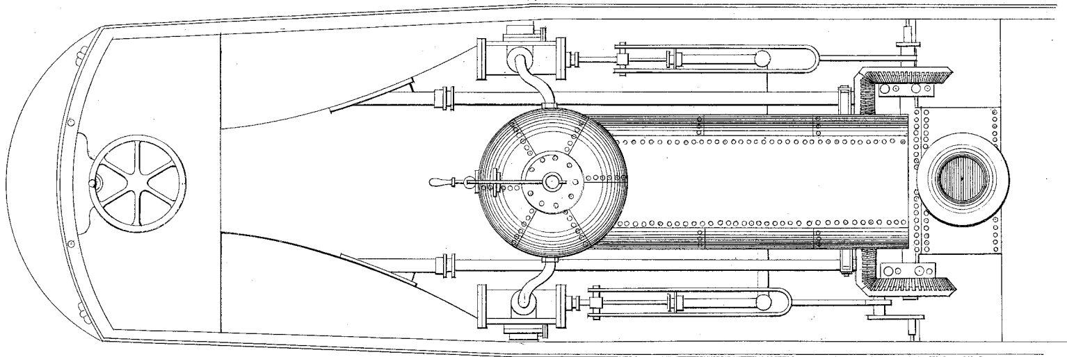
PLAN OF THE PIONEER.
