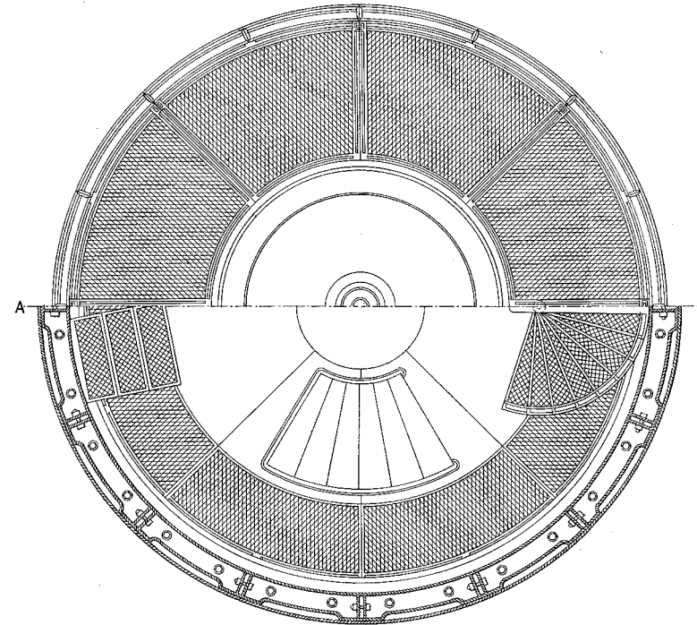
PLAN AT C D.
