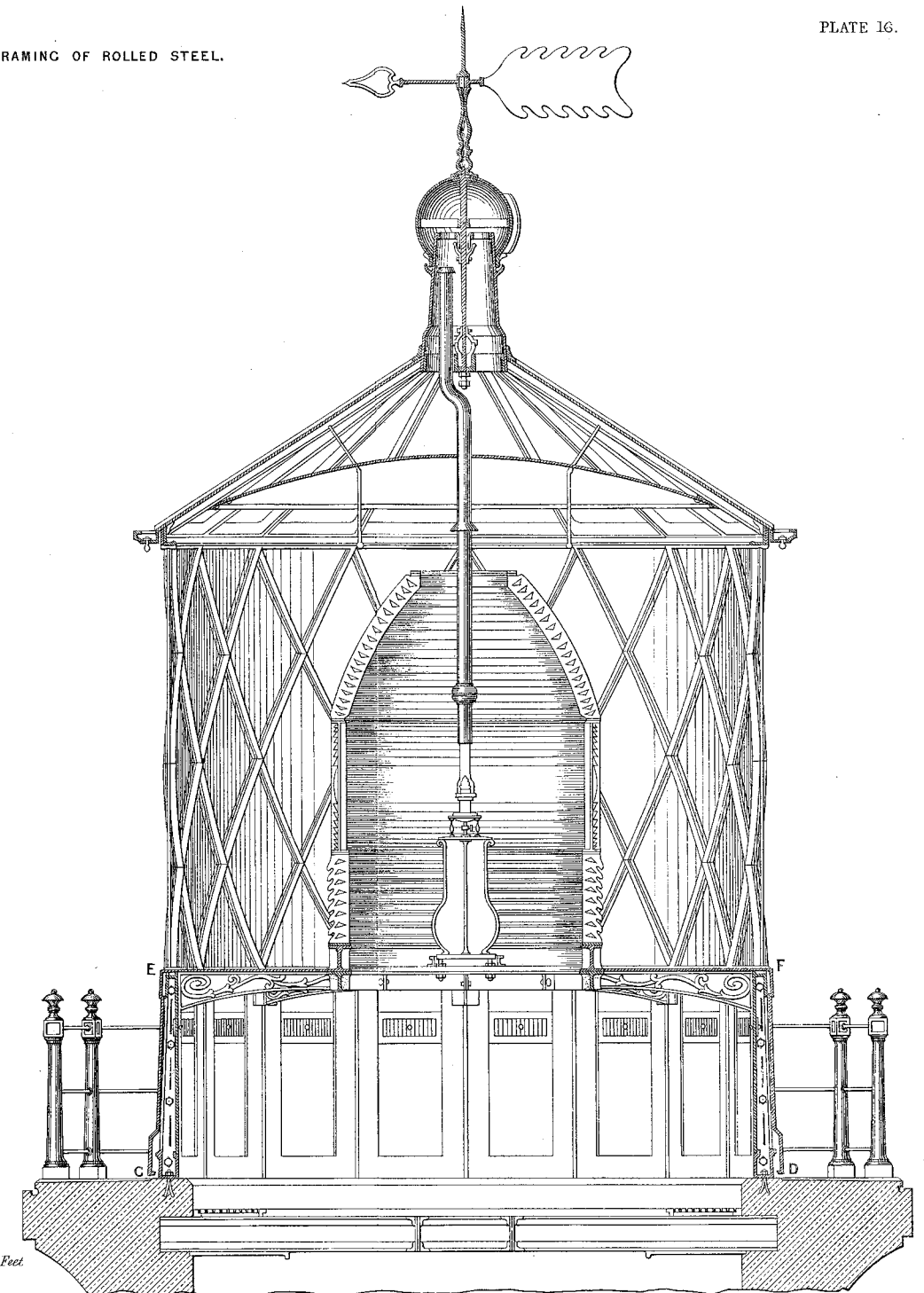
SECTION AT A B ON PLAN.
