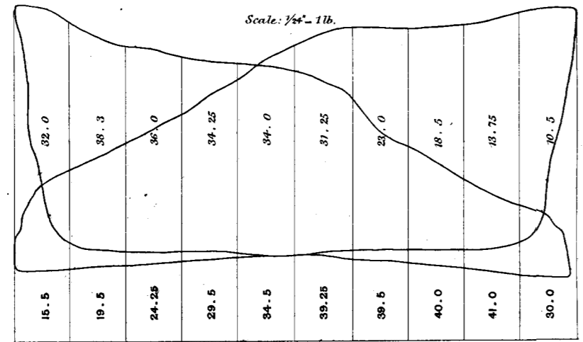
Official Trial at Skelmorlie, Sep r 11 th 1869. Speed, 11.1 knots per hour.
