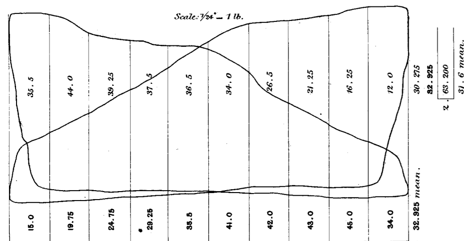
Official Trial at Skelmorlie, Sep r 11 th 1869. Speed, 11.1 knots per hour.
