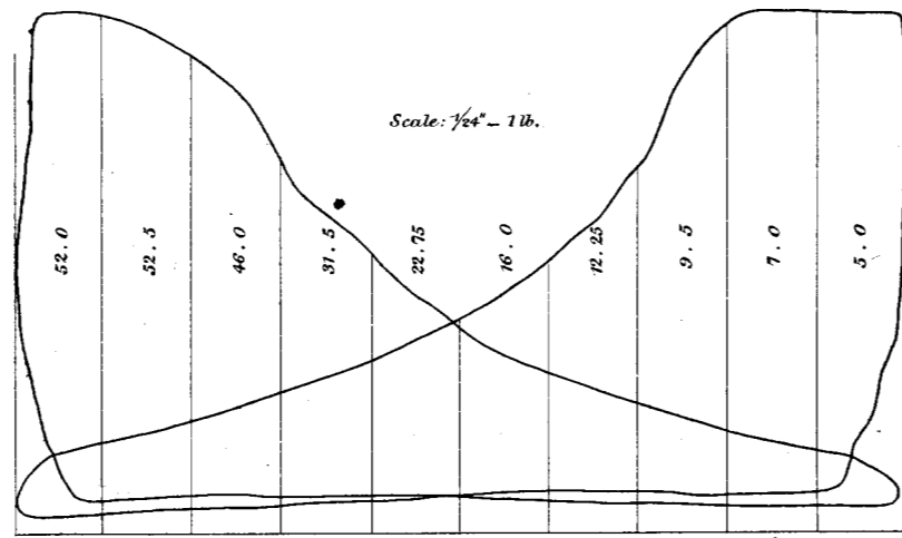
Official Trial, Cloch to Cumbræ, Sep r 14 th 1869. Speed, 9.6 knots per hour.
