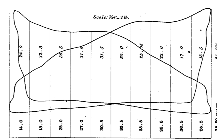
Official full power Trial at Skelmorlie, Jan r 4 th 1870.
