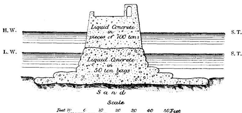
ABERDEEN HARBOUR.—PROPOSED EXTENSION OF NORTH PIER.
