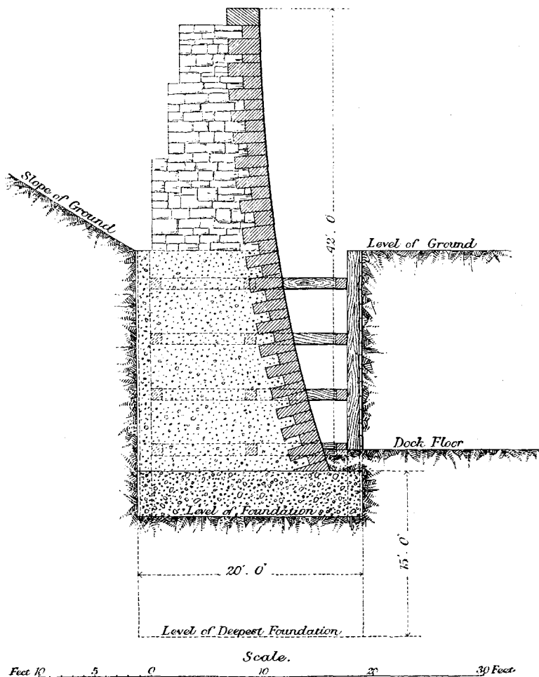
BRISTOL PORT AND CHANNEL DOCK.—SECTION OF EAST WALL.
