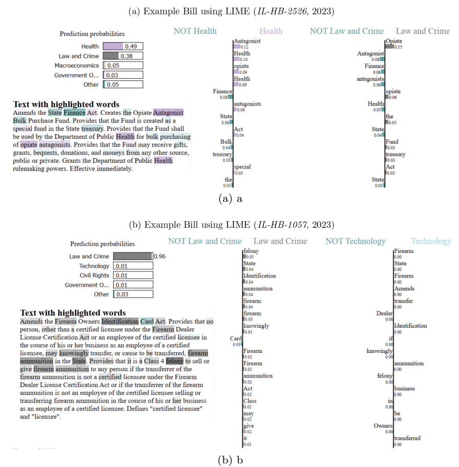
Figure 7: Explaining model predictions for example bills from Illinois.
