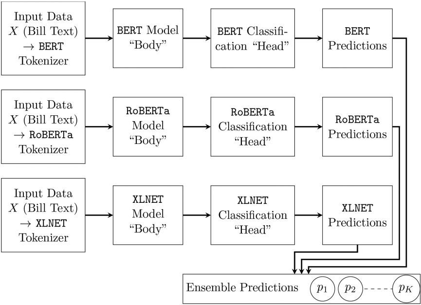
Figure 1: Ensemble model architecture. Notes: In a multi-class classification task, \sum_{k \in K} p_k = 1 , and the maximum p_{k, k \in K} is taken to be the model’s prediction for the bill’s topic, \hat{y} . In a multi-label classification task, the probabilities need not sum to 1. For either classification task, the 1024-dimensional document embedding generated by the RoBERTa-large model “body” forms the input for the classification “head,” which is itself a deep neural network. The model output is technically the output layer of the classification head, but the head is decomposed in this way to illustrate the specific form of the output.
