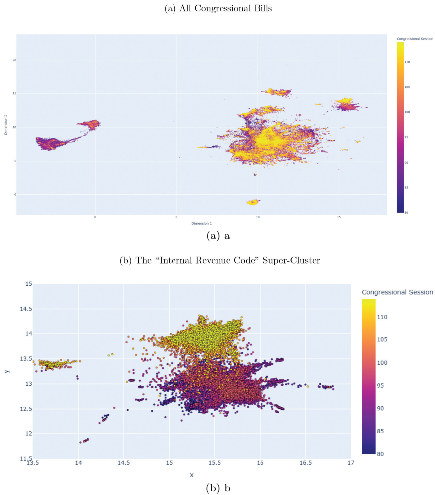
Figure 6: “Topic Drift” in congressional bills (80 th –114 th Congresses).
