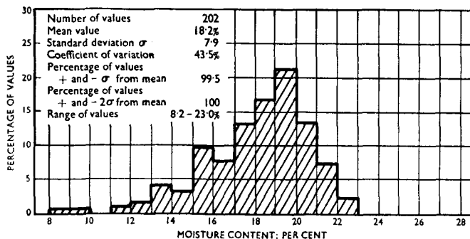
FIG. 50.—SOUTHEND AIRPORT. MOISTURE-CONTENT HISTOGRAM FOR NEW CEMENT-STABILIZED BRICK-EARTH PAVEMENTS
