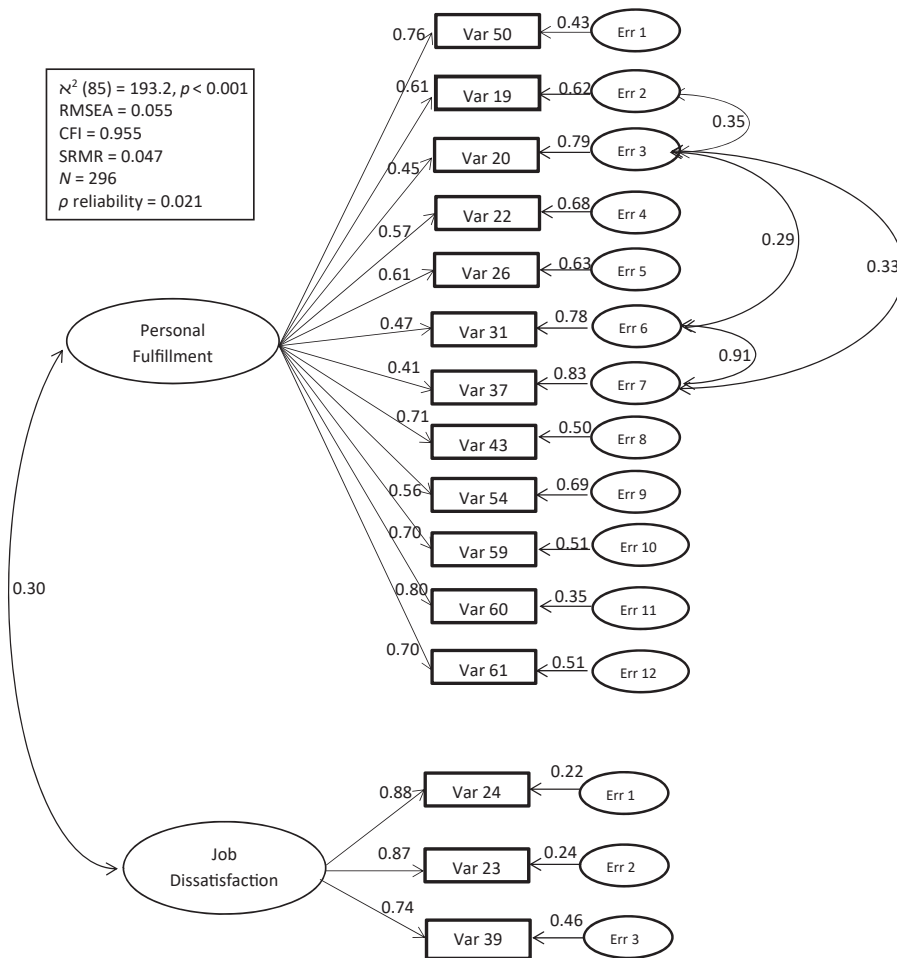
Figure 1. Two-factor CFA model
