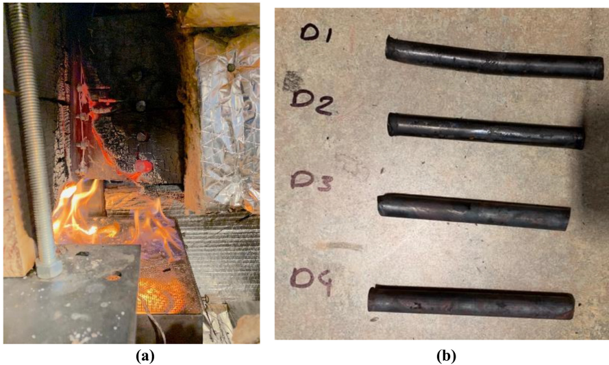
Plate 9. FP test images: (a) embedment failure of the beam at the lower dowel location and (b) bending of the dowel 1 (D1) at the end of FP test
