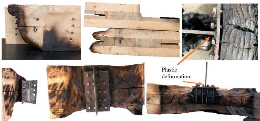
Plate 10. Residual section of the CLT beam-to-girder assembly after the fire-performance test
