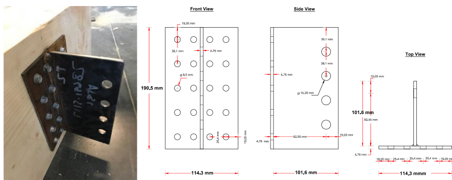
Figure 2. Attached T-shaped welded steel connection to the CLT Beam and its geometry
