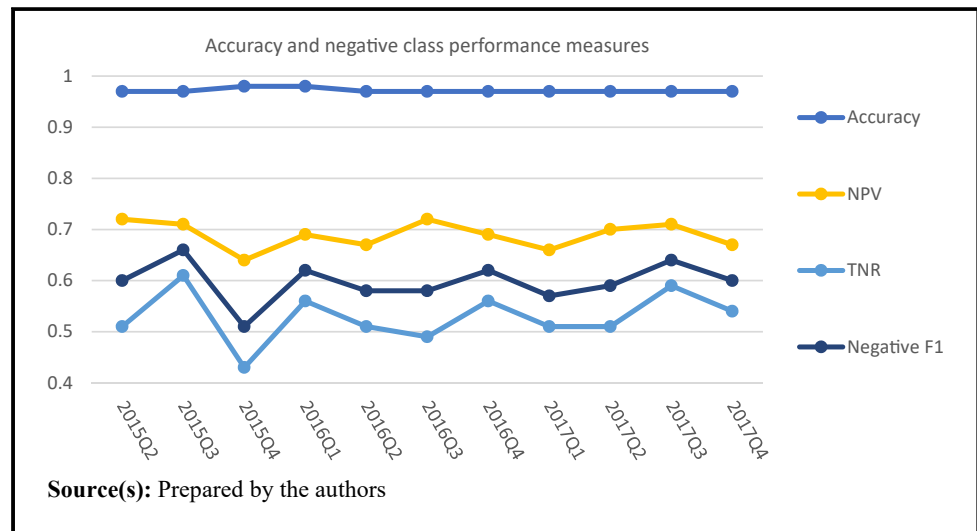
Figure 3 Accuracy versus performance measures for the negative class
