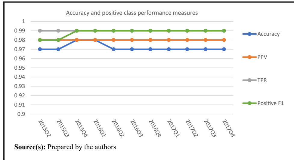
Figure 2 Accuracy versus performance measures for the positive class
