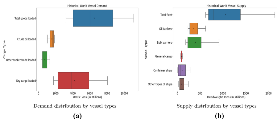
Figure 1. Descriptive statistics
