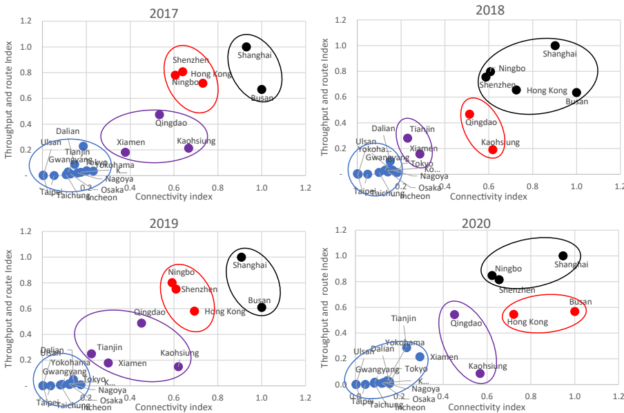
Figure 3. Categorizing ports based on FCM clustering
