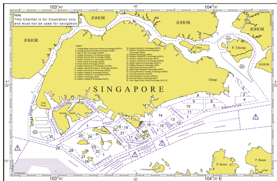
Figure 2. Anchorages and fairways in Singapore
