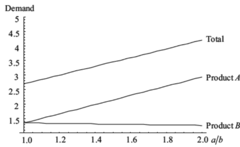
Figure 2. Demand rate based on the different product ratios a/b
