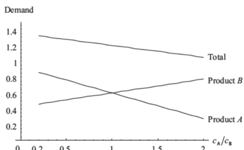
Figure 4. Demand according to different ratios c_A(\otimes)/c_B(\otimes)
