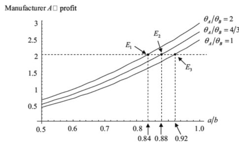
Figure 3. Profit of Producer A according to ratio a/b , \theta_A(\otimes)/\theta_B(\otimes)
