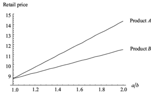
Figure 1. Retail sales price based on the different product ratios a/b
