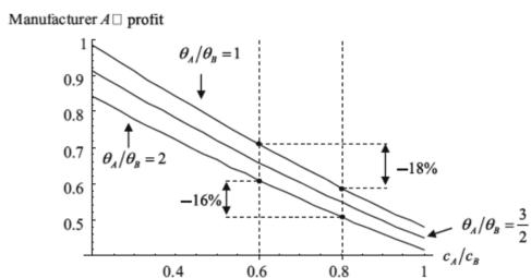
Figure 5. Profit of producer A according to ratio c_A(\otimes)/c_B(\otimes) , \theta_A(\otimes)/\theta_B(\otimes)
