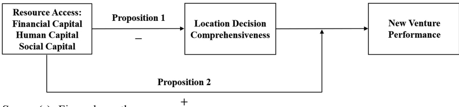
Figure 1. Theoretical model
