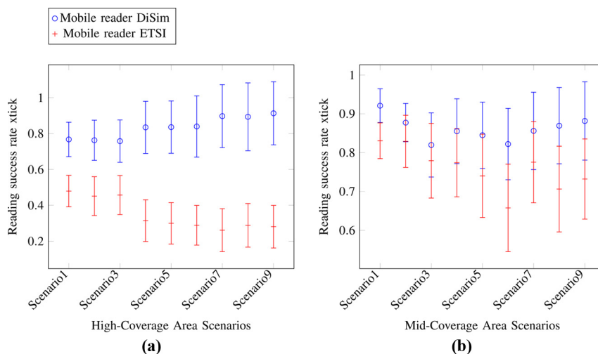
Notes: (a) Average reading success rate for high-coverage area; (b) average reading success rate for mid-coverage area
