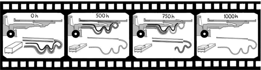
Figure 7. Animation showing how to optimize the changeover cycles of harnesses in-between complete bundle rebuilds
