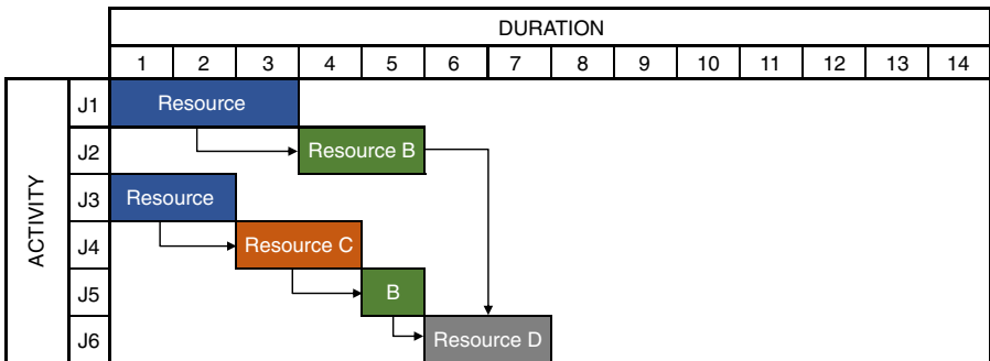
Figure 4. Schedule of activities with reduced durations
