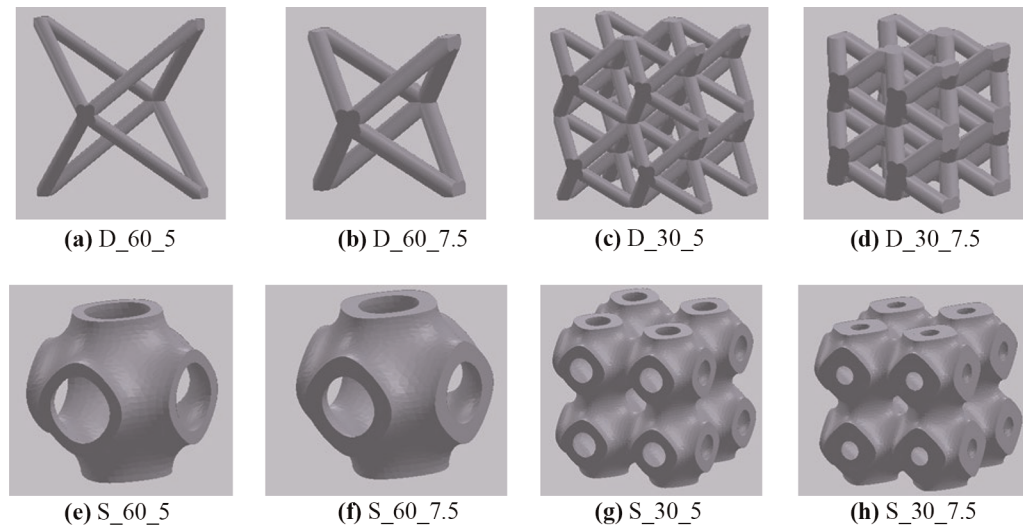
Figure 5 Lattice structure samples as a function of shape – cell dimension – node thickness
