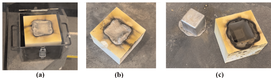
Figure 8 SP2 main steps: casting (a); cooling (b); and cube extraction (c)
