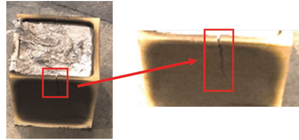
Figure 9 Crack formation during the cooling step of the mold with a 5 mm wall thickness
