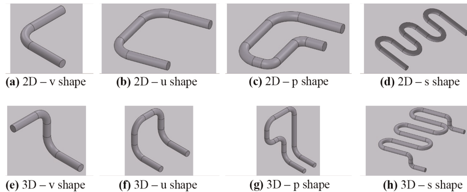
Figure 4 Demonstrators design for CP.2
