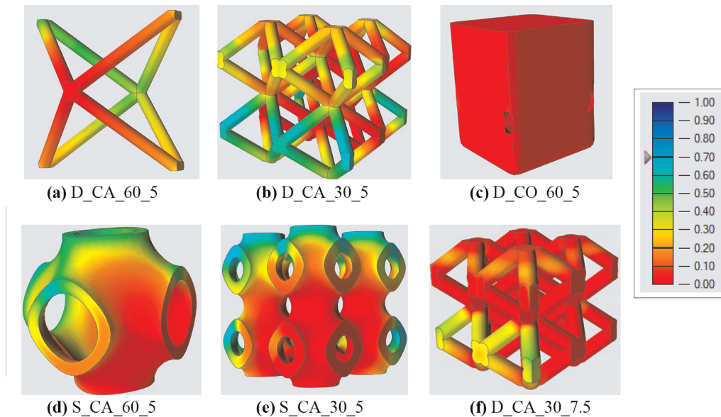
Figure 12 Volume fraction analysis most significant results
