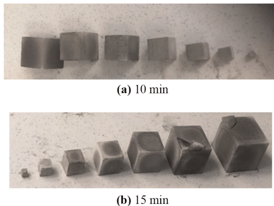
Figure 7 Set of cubes at the end of the SP.1 test
