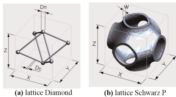
Figure 4 Demonstrators design for CP.2
