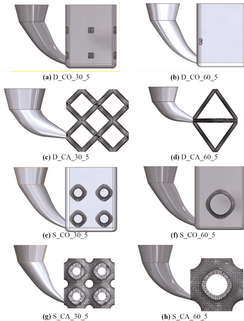
Figure 6 Negative design of the molds as a function of shape (D, S) function (CO, CA) cell dimension (30, 60) and node thickness (5)
