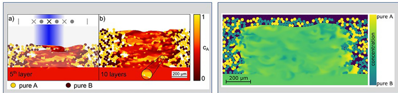
Figure 15 Left: 2D lattice Boltzmann (LB) multilayer simulation of a multimaterial PBF process using SAMPLE2D, reprinted from Scherr et al. (2020) : (a) the electron beam acting on the fifth layer is shown in blue; (b) the final composition profile after ten layers. Right: simulation result using SAMPLE2D taken from Küng et al. (2021) , concentration distribution after an EBM process
