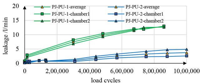
Figure 9 Comparison of leakage flows in AM-based RVAs with PU seals and PJ housings
