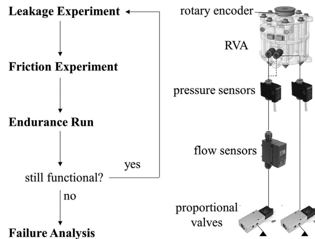
Figure 7 Overall testing procedure and hardware setup for the quality assessment of AM-based RVAs
