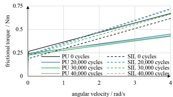
Figure 13 Dependence of friction on the number of load cycles for AM-based RVAs with SLS housings and PU (solid lines) or SIL (dashed lines) seals
