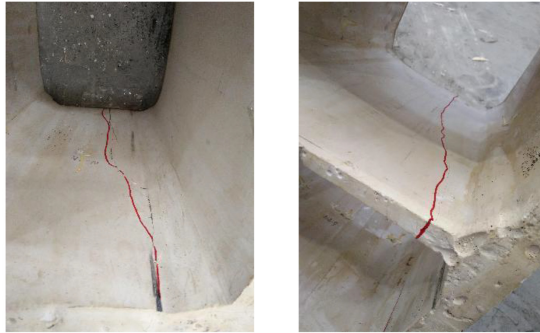
Cracked segment of lining structure (12#)
