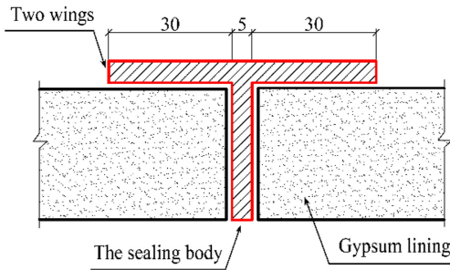
Special “T”-type rubber waterproof belt
