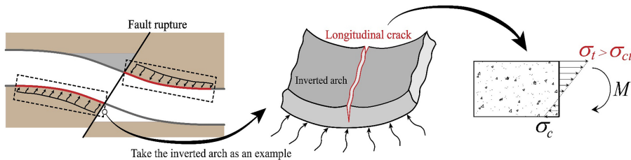
Figure 17. Schematic diagram of large eccentric tension damage on the cross-section of the tunnel structure
