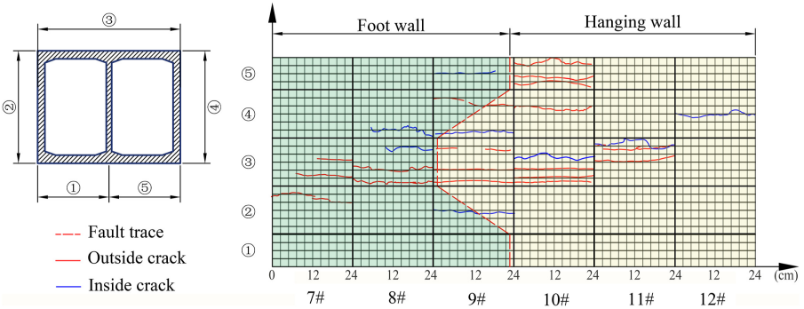
Figure 21. Tunnel crack expansion diagram
