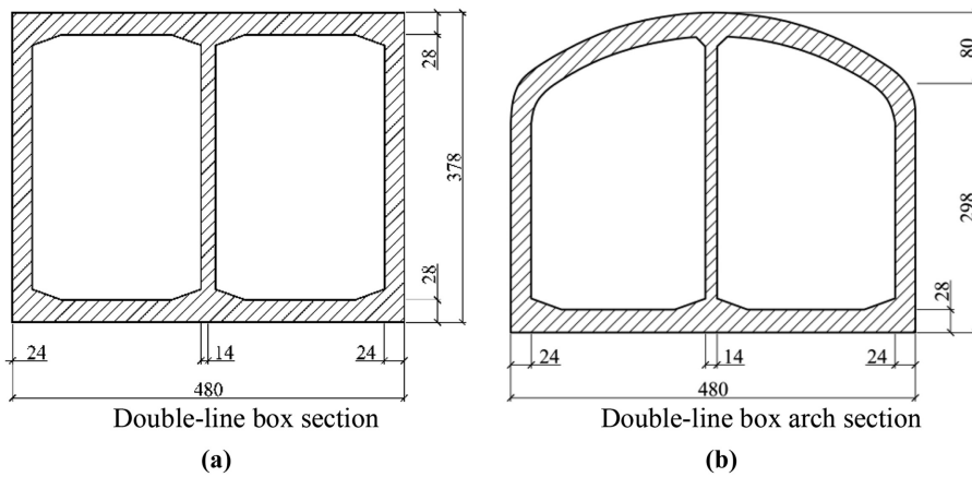
Figure 7. Size of the cross sections (unit: mm)
