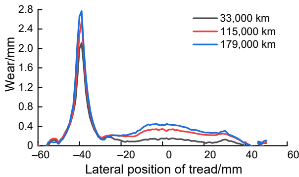
Typical tread wear distribution
