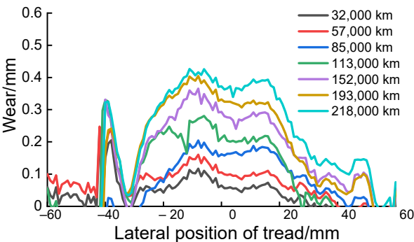
Typical tread wear distribution (c)
