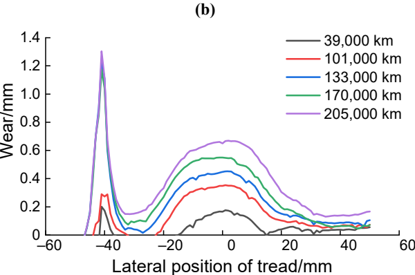
Typical tread wear distribution
