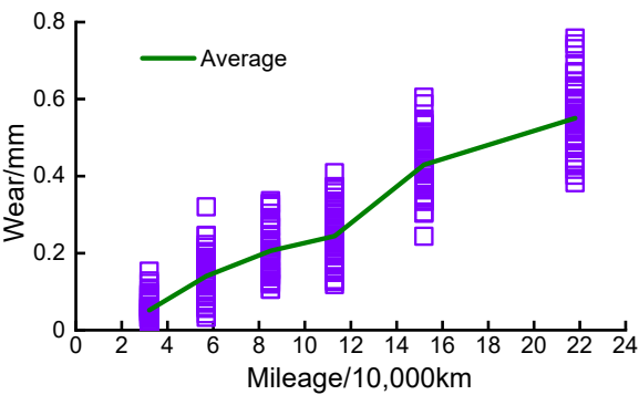
Tread wear changing with service mileage (a)
