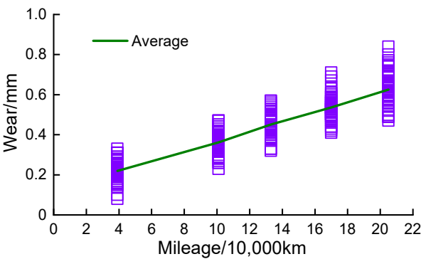
Tread wear changing with service mileage
