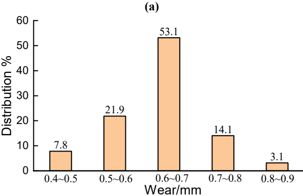
Statistics of tread wear at the end of a reprofiling cycle
