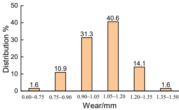
Statistics of tread wear at the end of a reprofiling cycle
