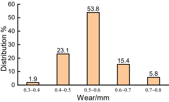
Statistics of tread wear at the end of a reprofiling cycle (b)
