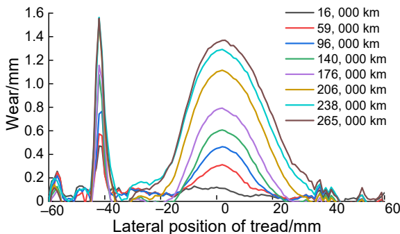
Typical tread wear distribution
