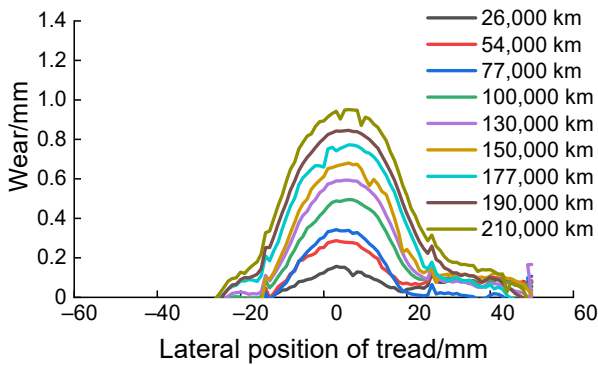
Typical tread wear distribution
