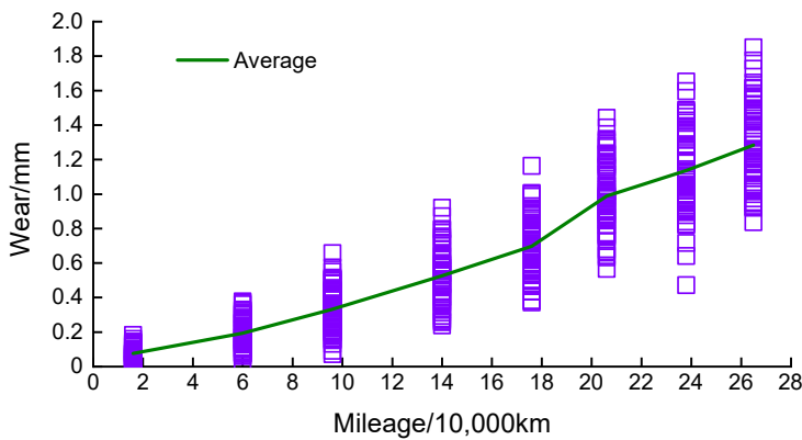
Tread wear changing with service mileage
