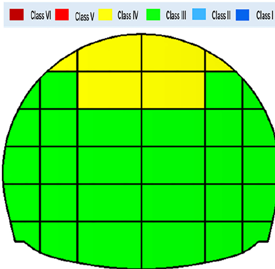
D2K584+320 section of Xiangjiawan Tunnel
