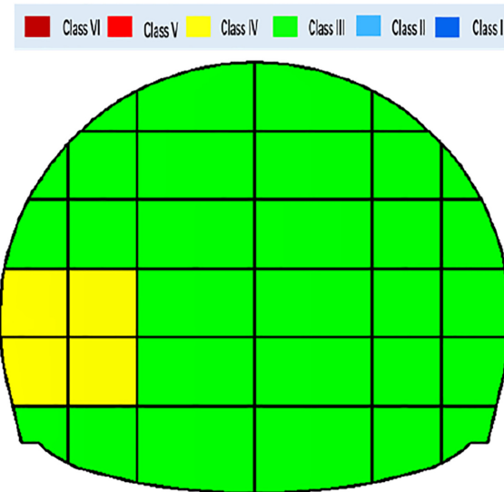
DK532+553 section of Chufeng Tunnel
