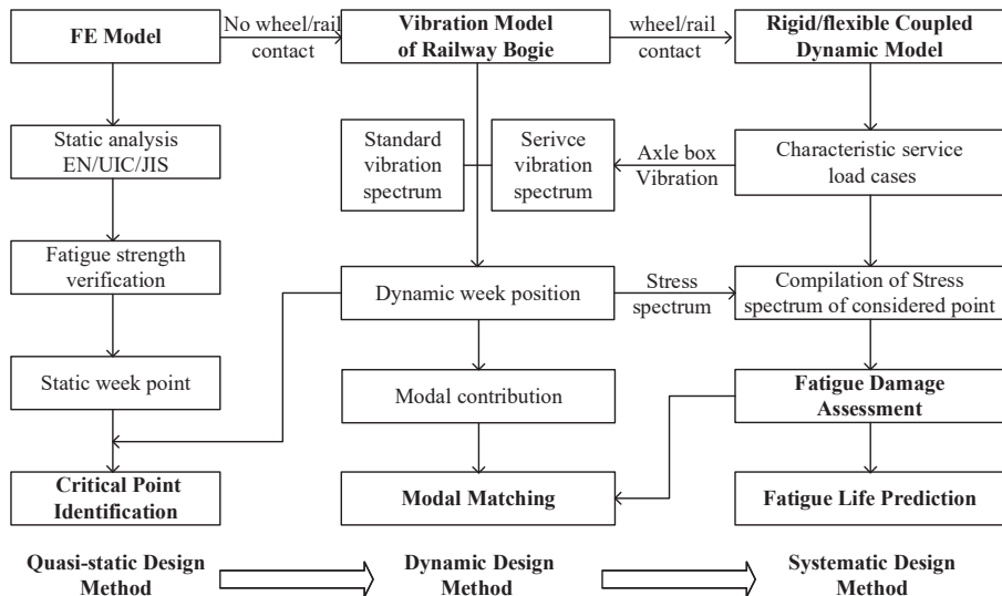
Figure 22. A systematic design method for vibration fatigue of railway vehicle
