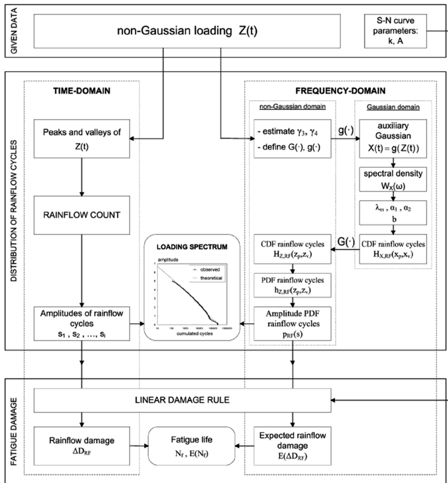
Figure 20. The non-Gaussian TB method together with the time domain method for the case of a non-Gaussian loading
