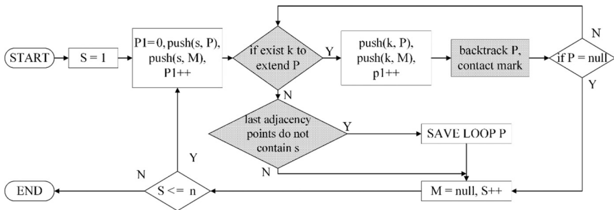
Figure 7. The flow chart of the amended Tarjan algorithm
