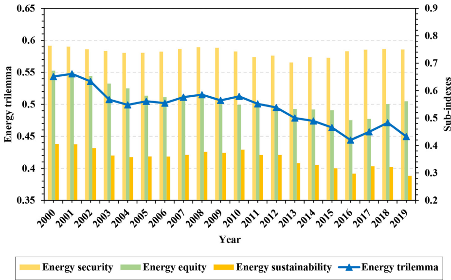
Figure 2. Time-trend chart of the ET and its three sub-indexes in China for the period 2000–2019
