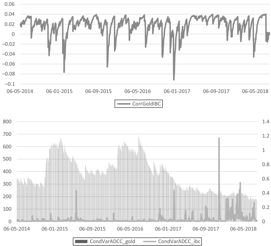
Figure 8. Volatility of IBC and gold (lower panel) and a conditional correlation between the assets (upper panel) Source: Authors.
