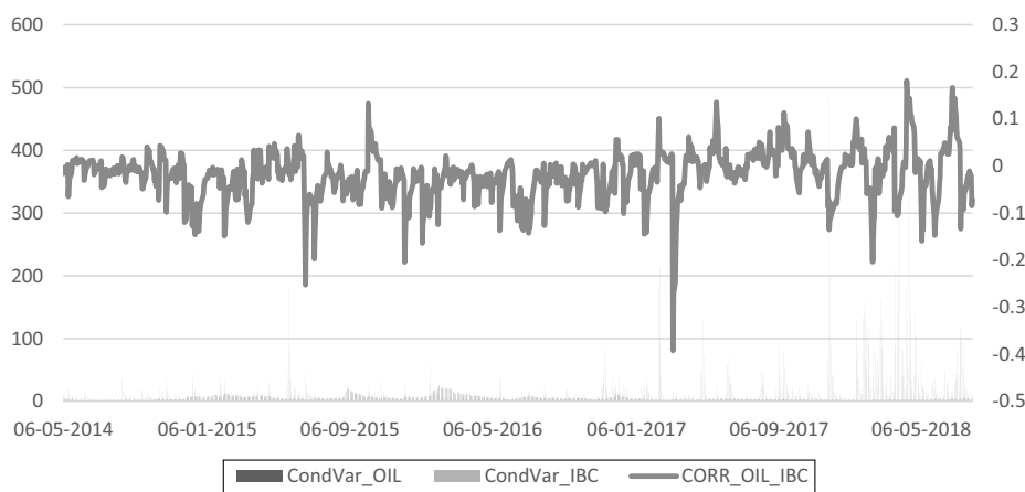
Figure 9. Volatility of IBC and oil (left axis) and a conditional correlation between the assets (right axis)
