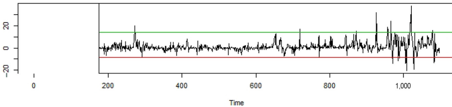
Figure 6. Threshold values for the TVAR model between IBC and OIL
