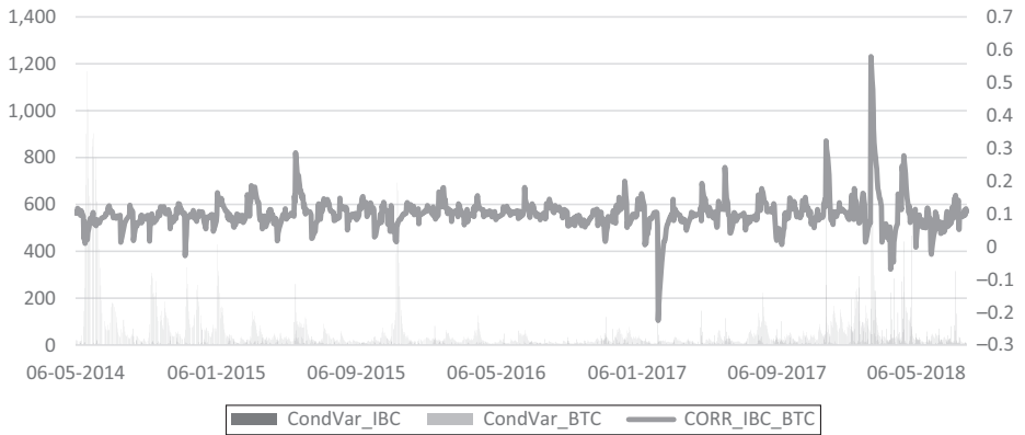
Figure 10. Volatility of IBC and BTC and a conditional correlation between the assets
