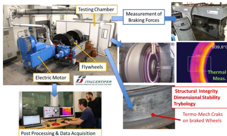
Figure 1 Dynamometric test rig for brake friction materials
