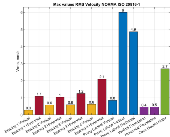
Figure 15 Measured velocity RMS on different measuring points (test at maximum speed, no flywheels installed)
