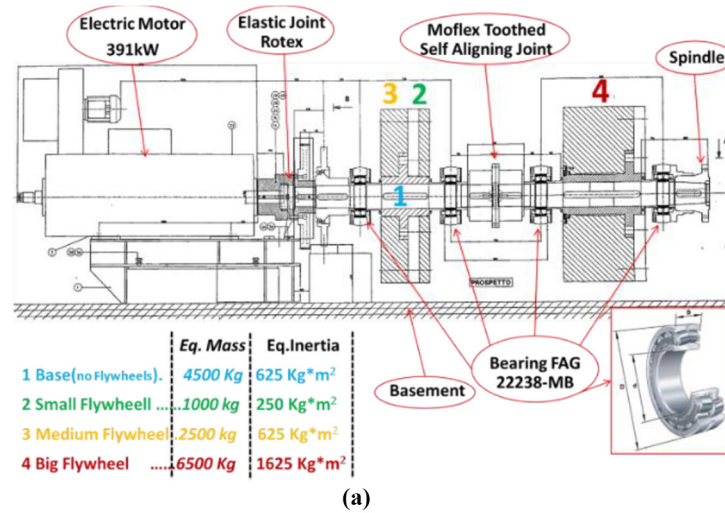
Figure 6 (a) Italcertifier test rig and (b) corresponding finite element model
