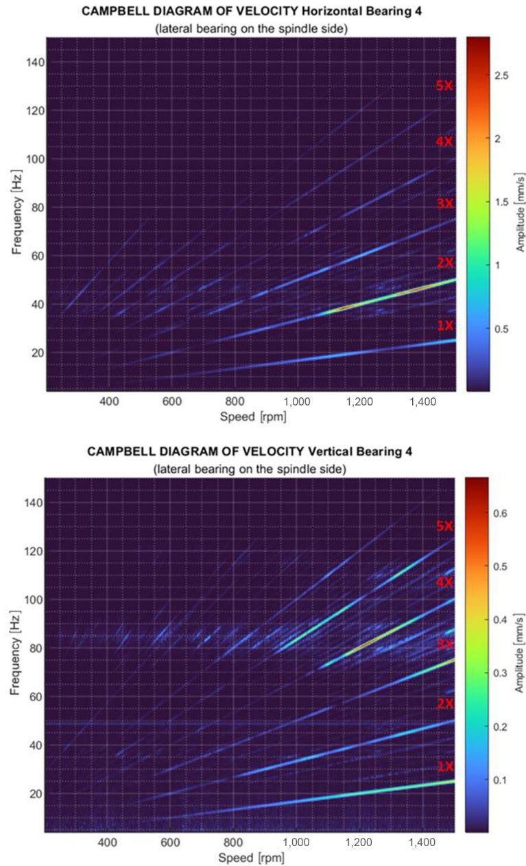
Figure 12 Spectrum of velocity rms v_{4rms}(\omega, \Omega) decomposed in terms of v_{4xrms}(\omega, \Omega) (top) and v_{4yrm}(\omega, \Omega) (bottom)
