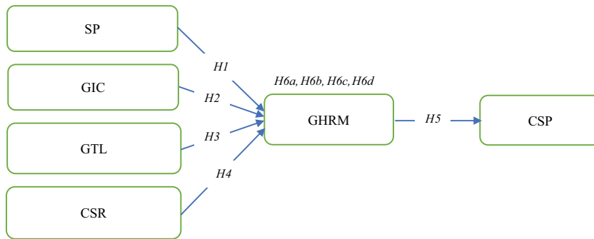
Figure 1. Research model
